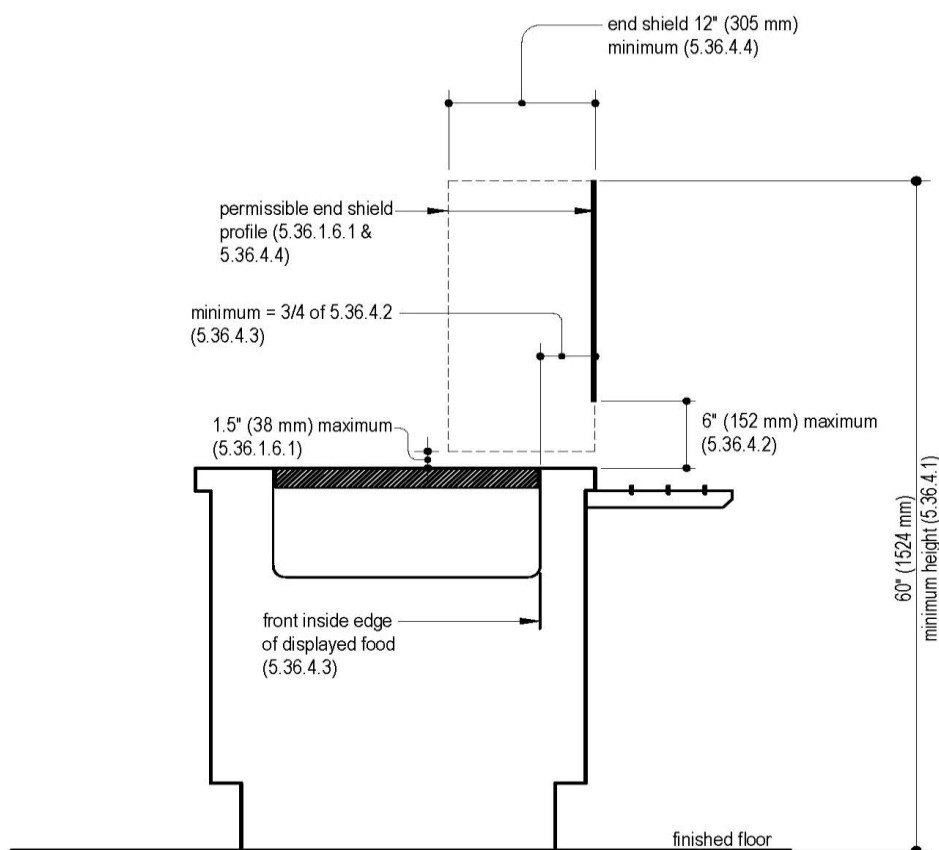
Figure 16B - Vertical Food Shield (5.36.4)
